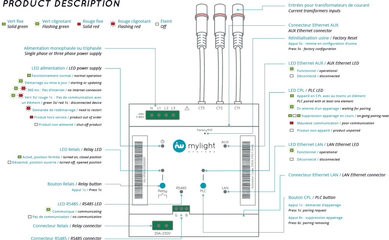
Figure 11. Description de la Smart Master G3
